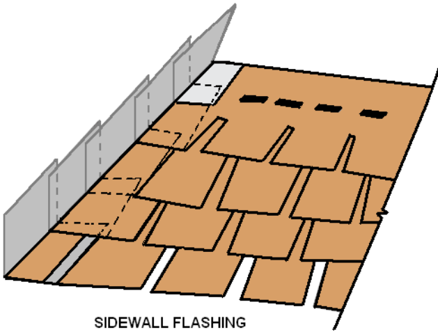
SIDEWALL FLASHING
